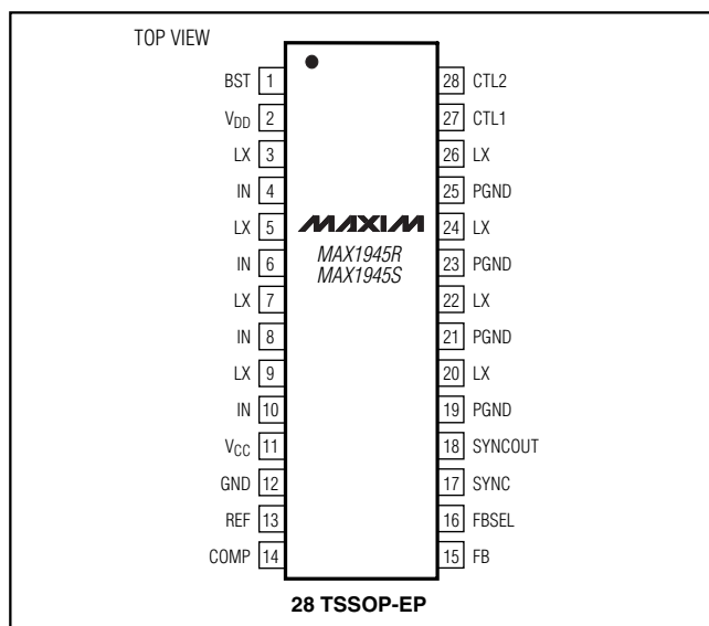
Pin Configuration
